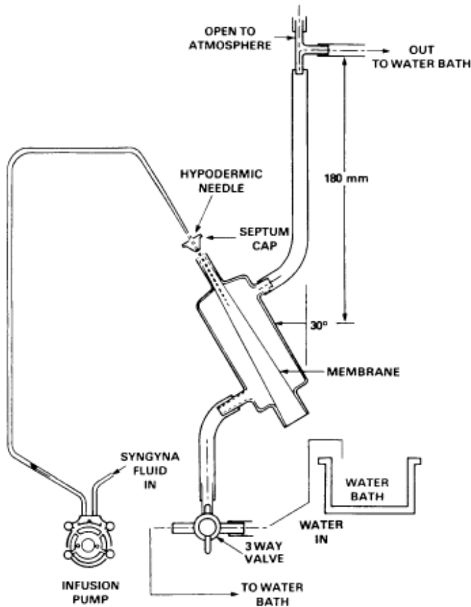
FIGURE 2—SYNGYNA TEST SET-UP
